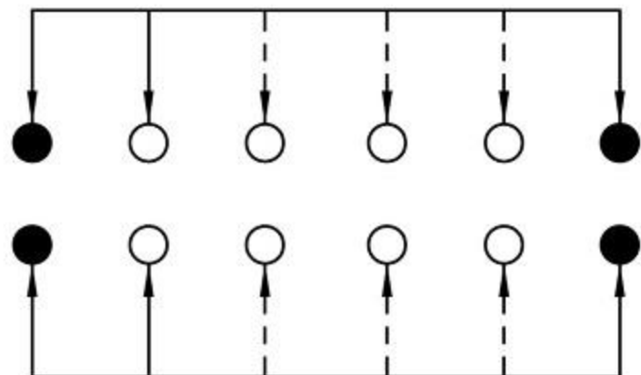
SCHEMATIC (NON-SHORTING)
